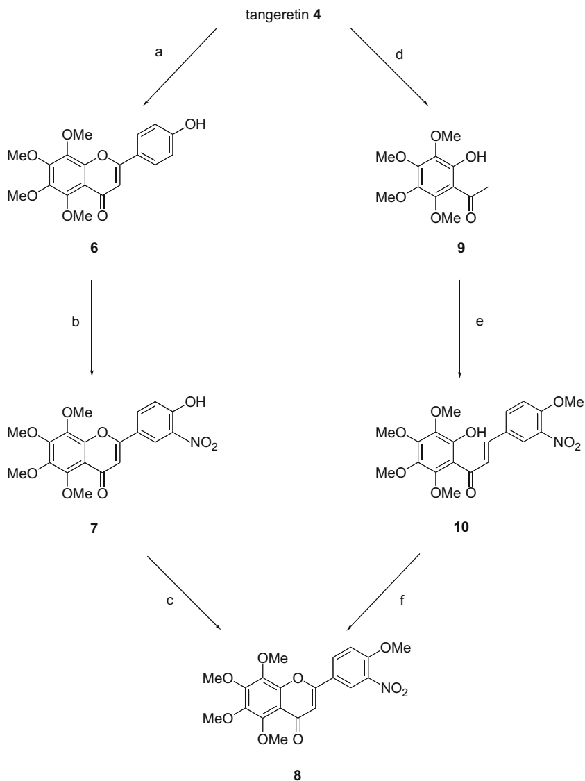
Scheme 1. Reagents and conditions: (a) Aspergillus niger , 70%; (b) 1 equiv \text{HNO}_3 , TFA, 0^\circ\text{C} , 0.5 h, 45%; (c) iodomethane, \text{K}_2\text{CO}_3 , DMF, rt, 1 h, quantitative yield; (d) EtOH–40% aq KOH, reflux, 5 h, 56%; (e) MeOH–50% aq KOH 10:1, 3-nitro-4-methoxybenzaldehyde, rt, 15 h, 60%; (f) \text{I}_2 , pyridine, 120^\circ\text{C} , 10 h, 52%.
