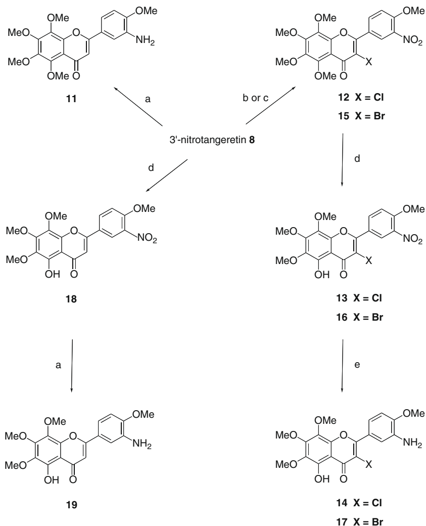
Scheme 2. Reagents and conditions: (a) \text{H}_2 , Pd-C 10%, DMF, rt, 3 h, 93%, ( 11 ), 95% ( 19 ); (b) NCS, \text{CH}_2\text{Cl}_2 -pyridine 4:1, rt, 48 h, 95%; (c) NBS, \text{CH}_2\text{Cl}_2 -MeOH 2:1, rt, 5 h; extraction then THF-NaOH N 1:1, rt, 0.25 h, 95%; (d) \text{AlBr}_3 , acetonitrile, 0 °C, then HCl 1 N, 50 °C, 0.33 h, 60% ( 13 ), 64% ( 16 ), 69% ( 18 ); (e) \text{SnCl}_2 , 2\text{H}_2\text{O} , MeOH, 60 °C, 14 h, 53% ( 14 ), 41% ( 17 ).
